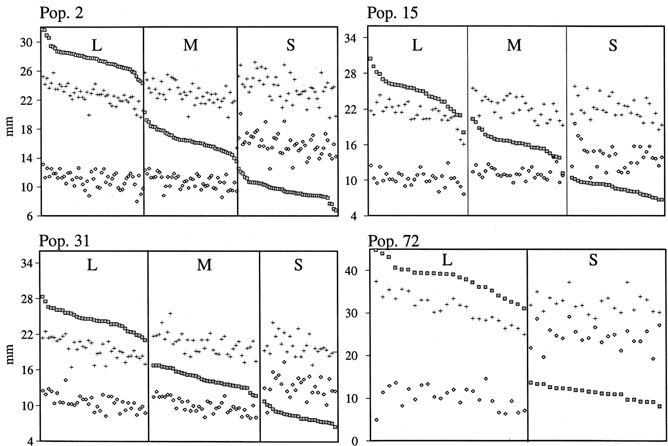
Fig. 1 Variation in the height of female and male sexual organs in four populations of Narcissus triandrus (style length \square , upper anthers +, lower anthers \diamond ). Individuals in each population are ordered by decreasing style length. Each anther height is the mean of the three anthers per level. Note that, in trimorphic populations, three distinct morphs are evident differing in the sequence in which anthers and stigmas are presented. Unlike most tristylous species, anther heights are similar in the L and M morphs. In the dimorphic population, the M morph is missing. Populations 2, 15 and 31 are trimorphic and population 72 is dimorphic for style length. Localities for the populations are 2 — Calera de León-1, Badajoz province, Spain; 15 — El Raso-1, Avila province, Spain; 31 — Alvares, Beria Litoral province, Portugal; 72 — Cedeira-1, La Coruña province, Spain.
